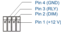
FIG. 7 RE-DM4 module connector
